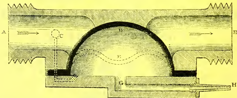
Fig. 2.—Full Size Section of the Valve or Patent Regulator.
