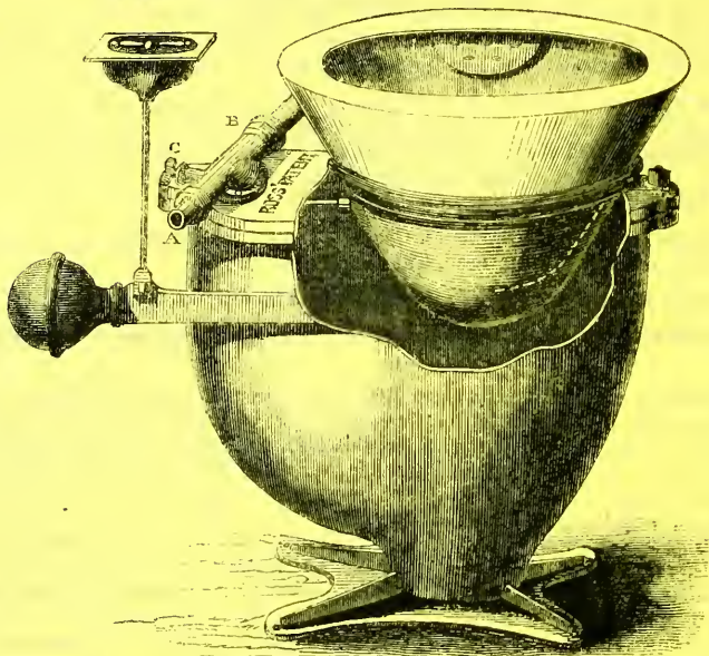
Fig. 1.—The ordinary Pan Water-Closet, with part of Trunk broken, to show mode of Working Valve.
