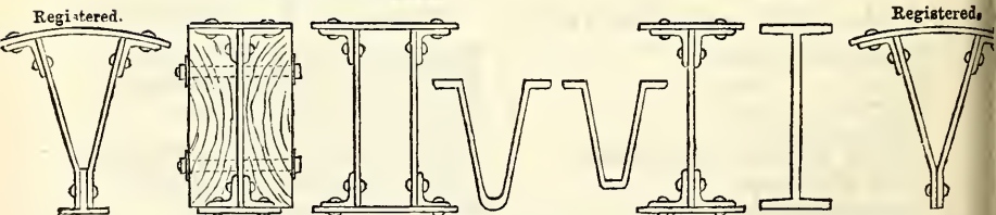
ROLLED MALLEABLE IRON JOISTS AND GIRDERS.
