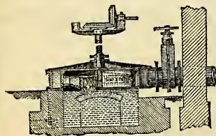
Turbine Water Wheel.
