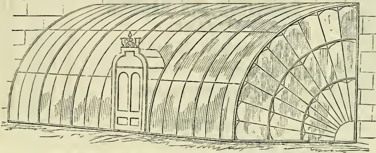
SPECIMEN OF ONE OF W. B. & CO.'S IRON AND GLASS HOHOUSES, 24 feet long, 12 feet wide, and 12 feet high. Prices, with and without Porch, £50 and £37, 10s. respectively, with underground foundations. No mason-work required.
