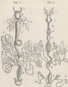
The organs of digestion in two different beetles. Fig. 1, a, garden beetle ( Carabus ). Fig. 2, a churchyard beetle ( Blaps ). a, the jaws and feelers, b, the head; c, c, the saliva vessels; d, the gullet, very short in Fig. 1; e, the crop, wanting in Fig. 1; f, the gizzard, wanting in Fig. 1; g, the stomach, large and convoluted in Fig. 1; h, h, h, the bile vessels long, and numerous; i, the small intestine; k, the blind gut; l, the vent; m, m, the excrementary vessels.
