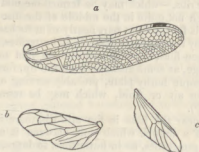
a , wing of dragon fly ; b , wing of bee ; c , wing of a house fly.
