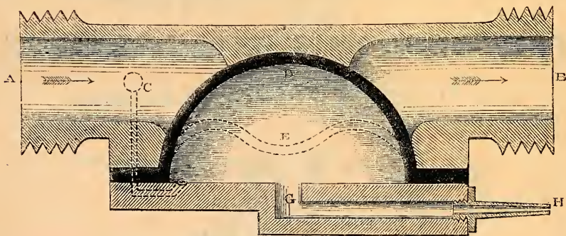
Fig. 2.—Full Size Section of the Valve or Patent Regulator.
