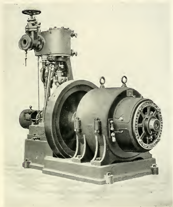
Small Direct Coupled "P.P.P." Steam Dynamo.
