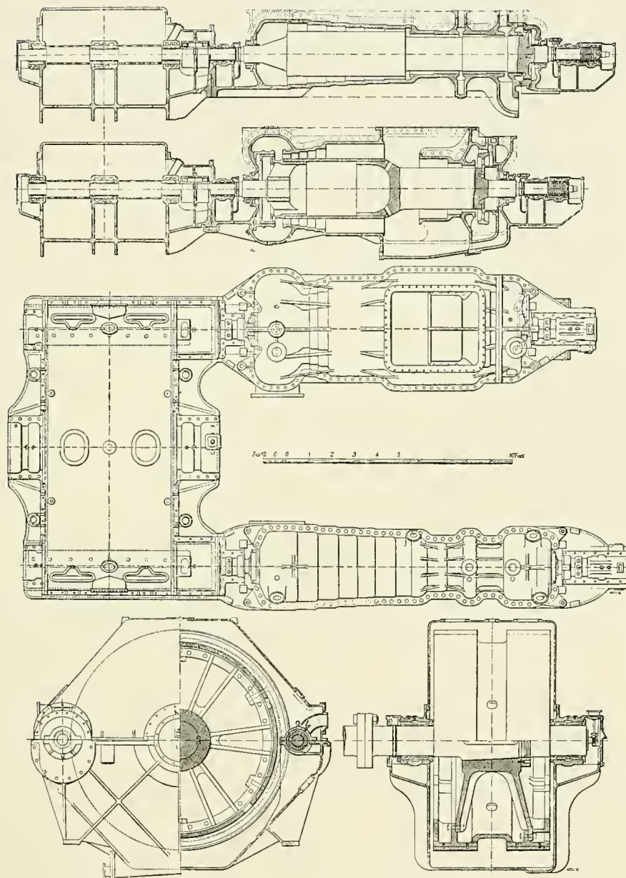
THE SINGLE-REDUCTION GEARED TURBINES OF THE " TRANSYLVANIA. "
