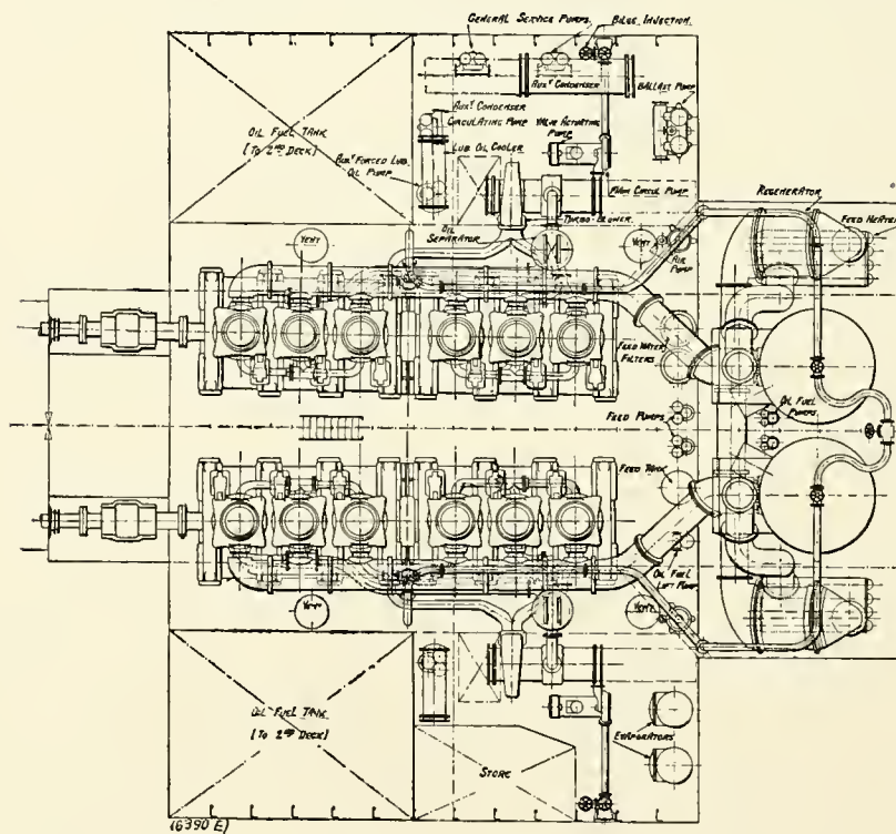
GENERAL ARRANGEMENT OF "STILL" ENGINES FOR TWIN-SCREW VESSEL.
