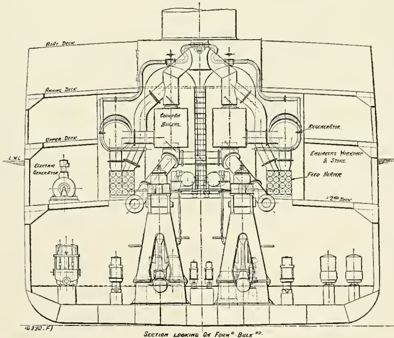
ARRANGEMENT OF "STILL" ENGINES, SECTIONS.
