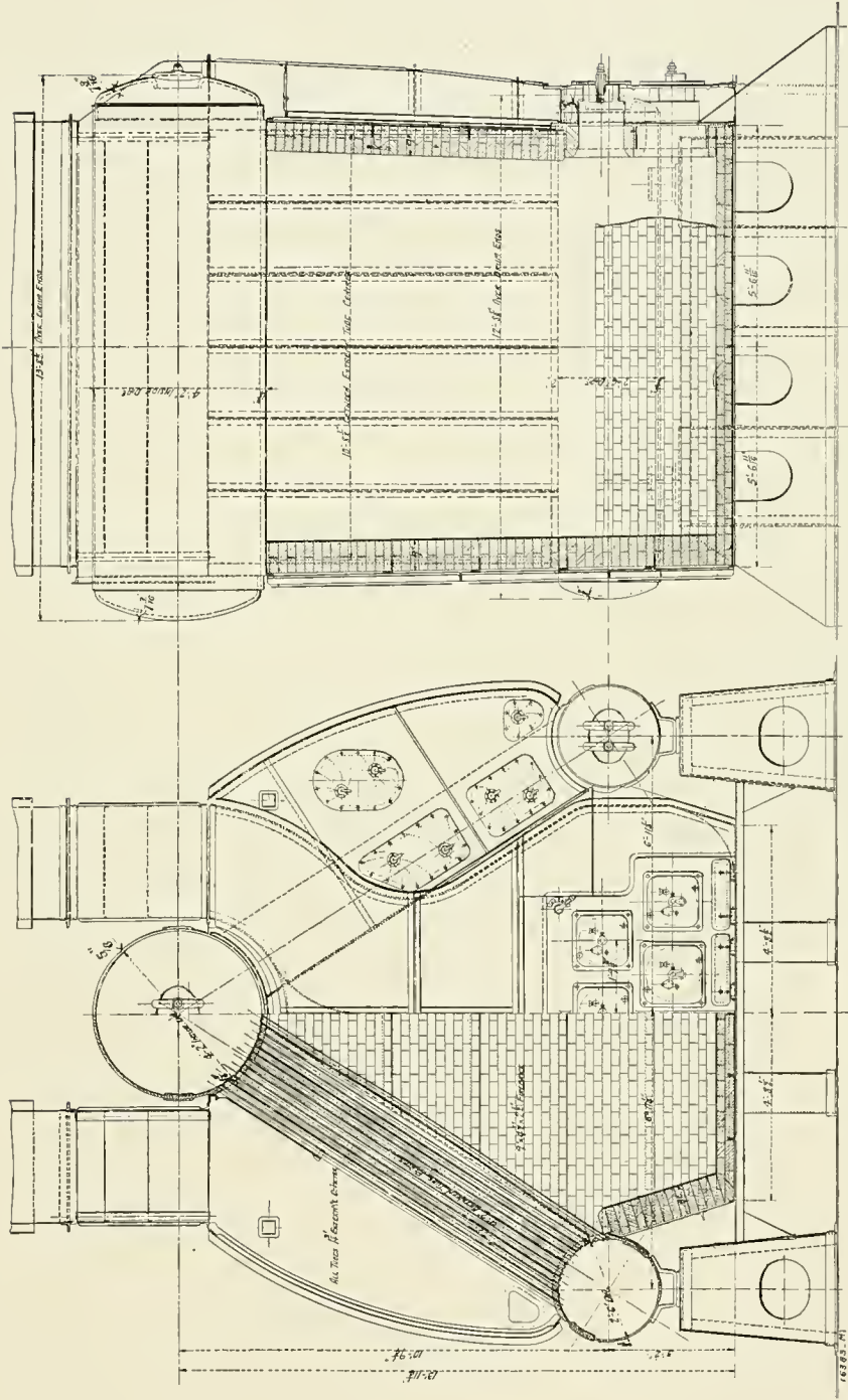
OIL-BURNING WATER-TUBE BOILER FOR A MERCHANT LINER.
